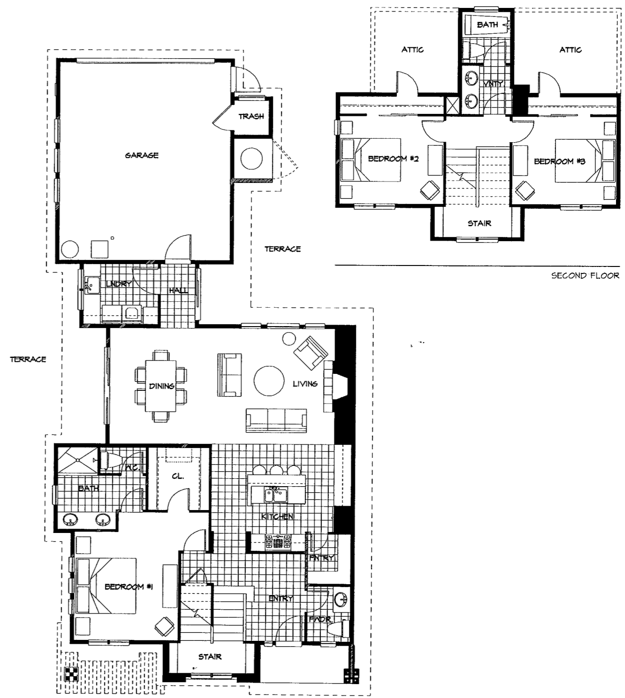
MERIWETHER 'C' 1,896 SF FIRST FLOOR
